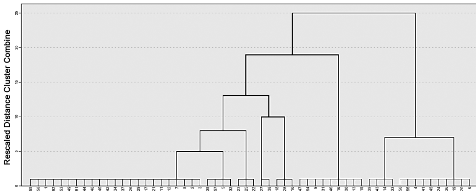
Figure 1. Dendrogram of firm clustering using the Average Linkage method
